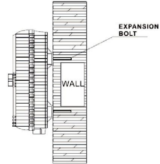
Wall mounted installation
